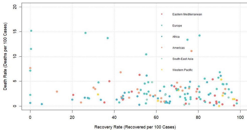
Death Rate vs Recovery Rate (Countries with >1000 cases)
