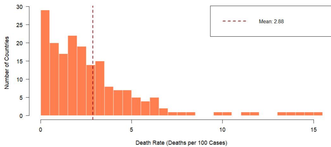
Distribution of COVID-19 Death Rates Across Countries
