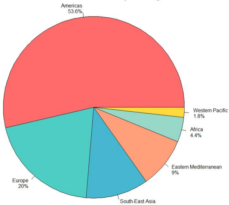
Distribution of Confirmed Cases by WHO Region
