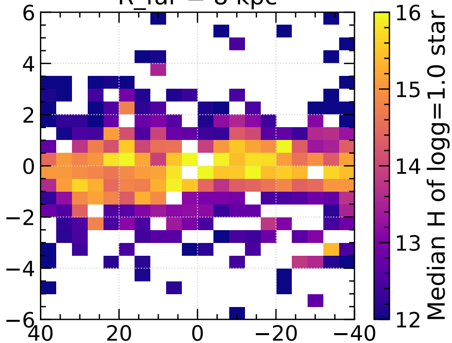
R_{\text{far}} = 8 \text{ kpc}
