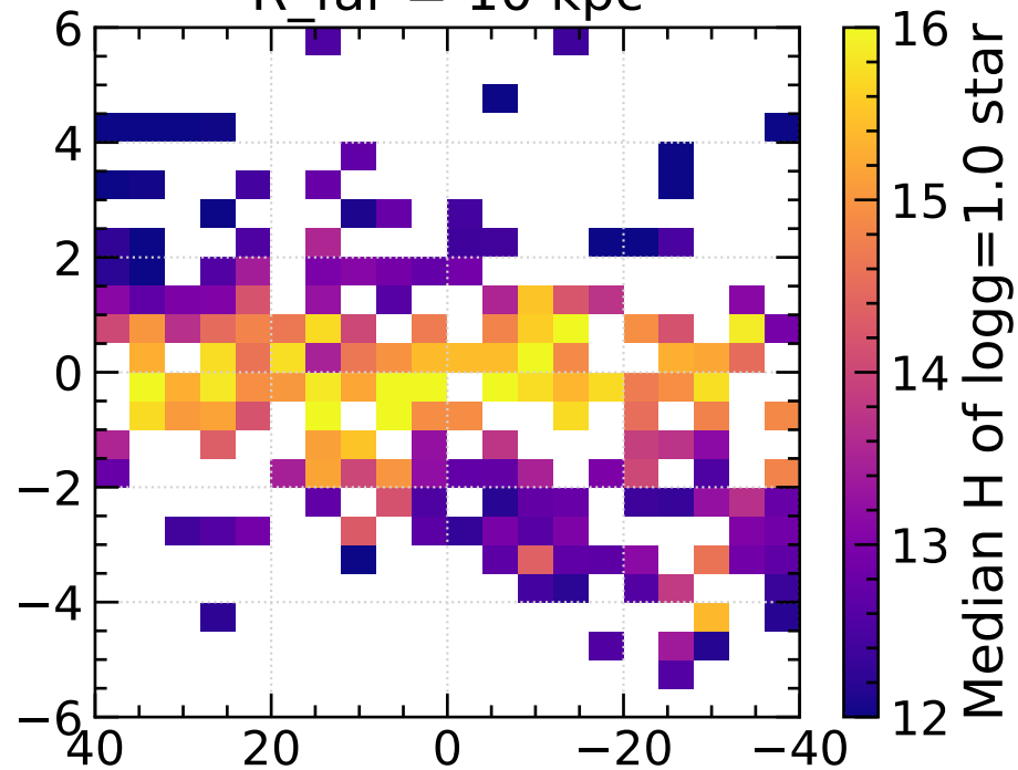
R_{\text{far}} = 10 \text{ kpc}
