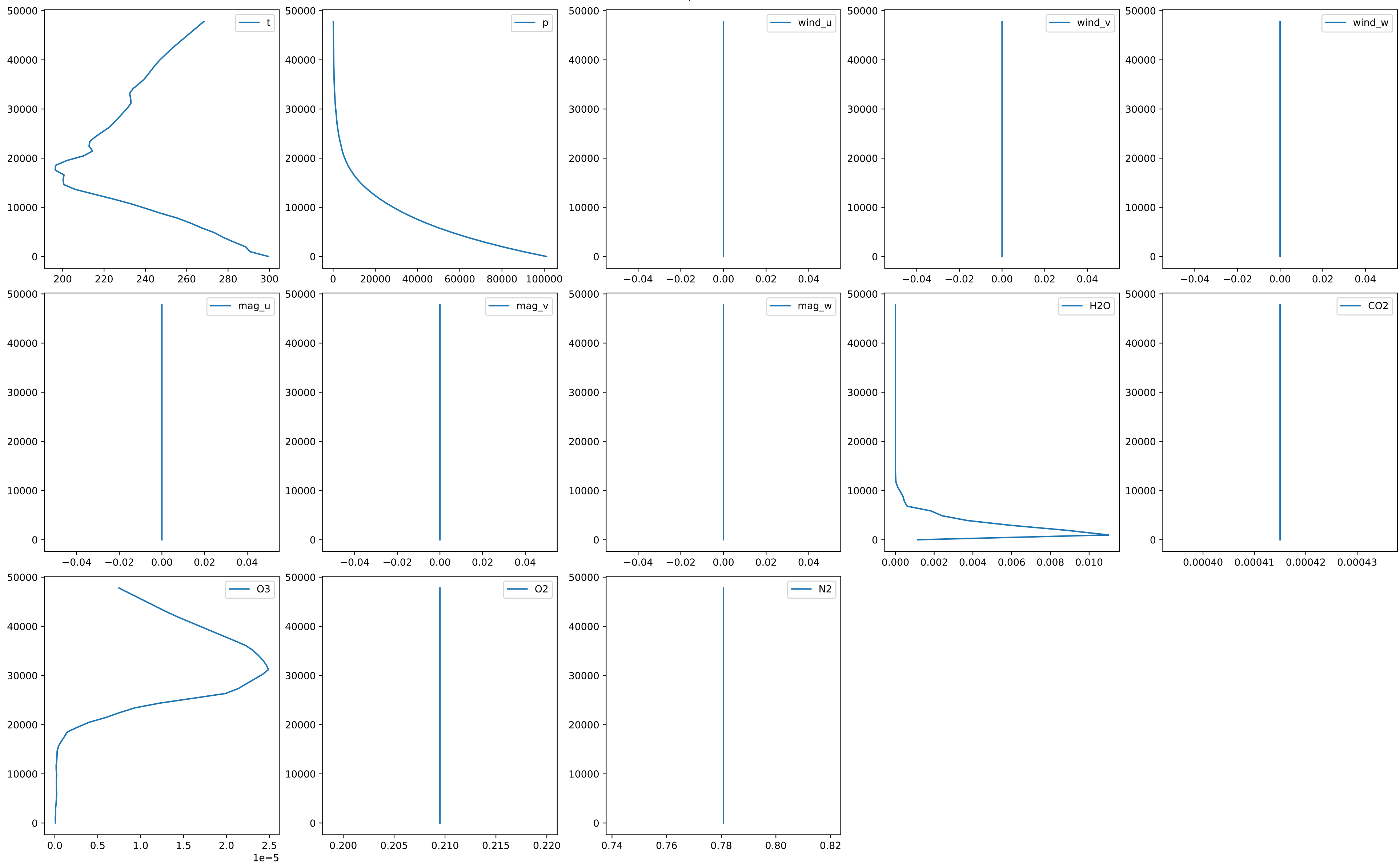
Atmospheric field
