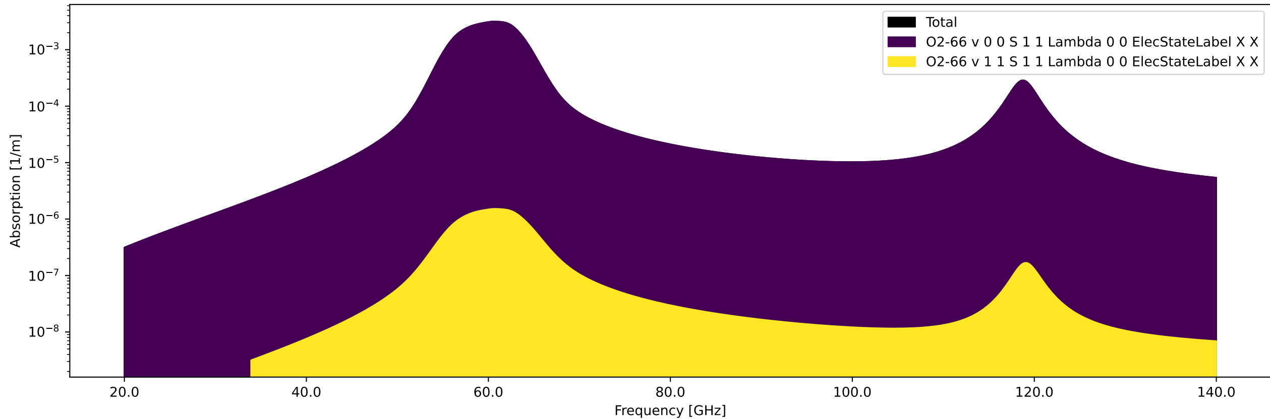
O 2 line-by-line absorption 20-140 GHz separated by bands
