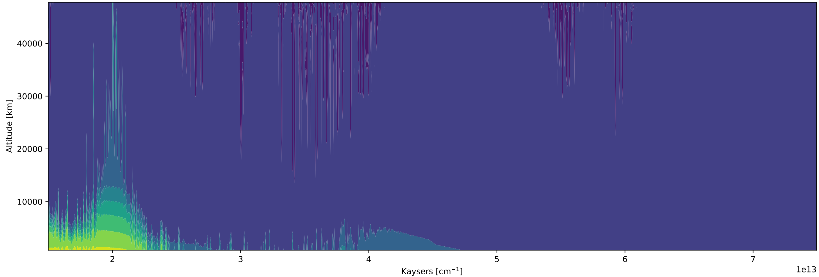
Downward diffuse spectral flux from DISORT
