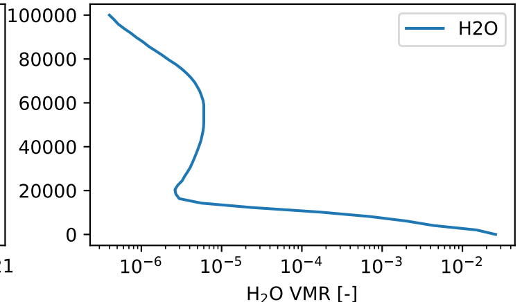
H 2 O VMR profile
