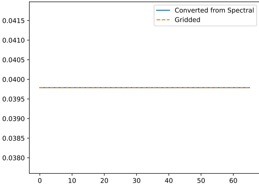
Henyeey-Greenstein phase function
