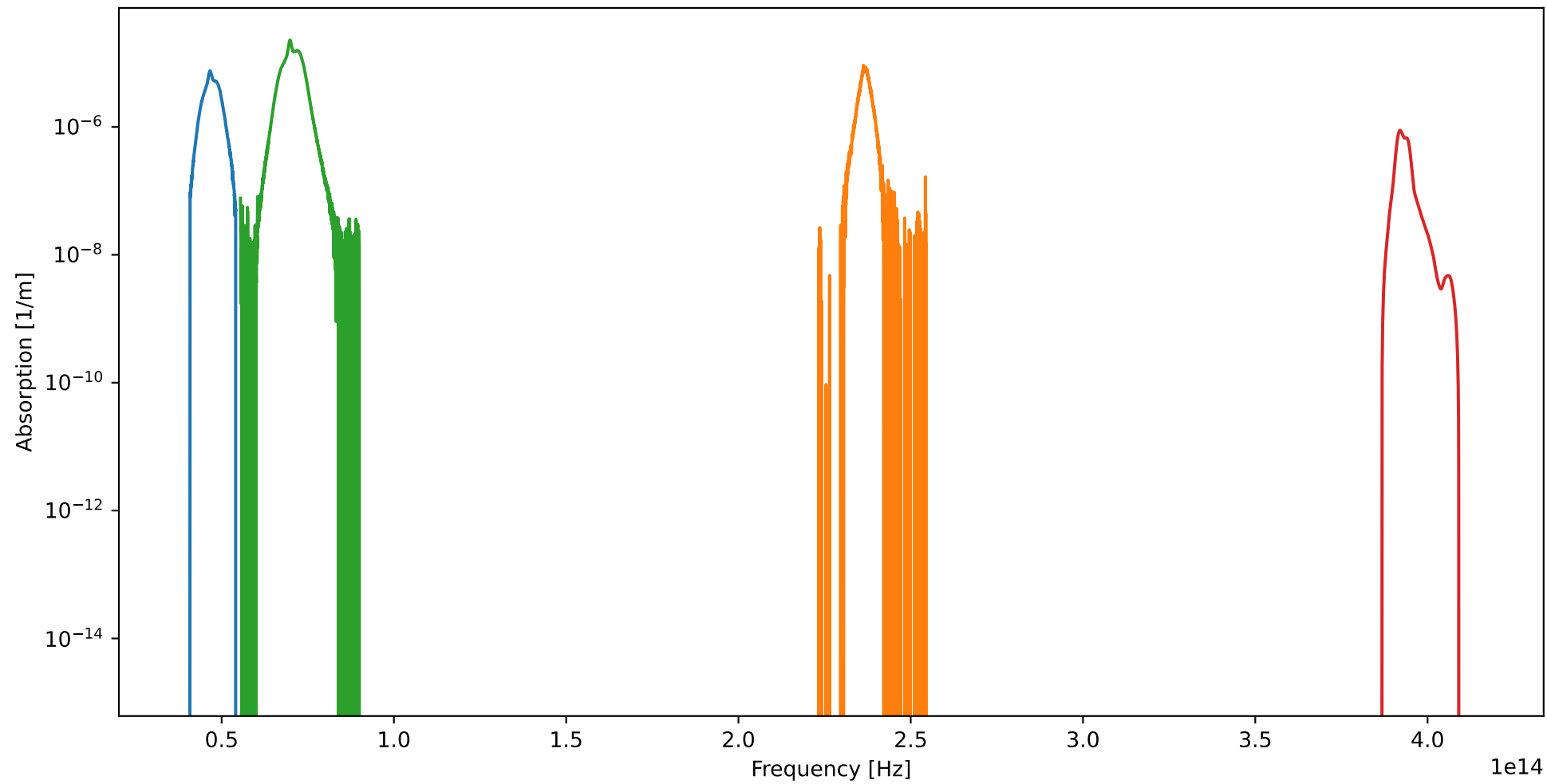
O 2 -N 2 Collision-induced absorption
