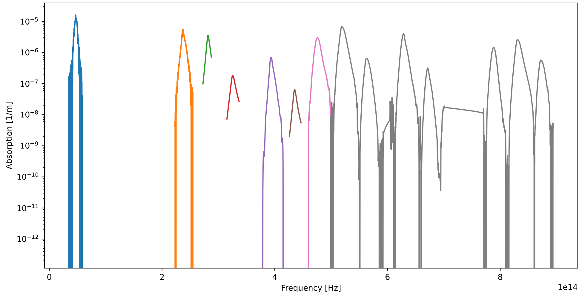
O 2 -O 2 Collision-induced absorption
