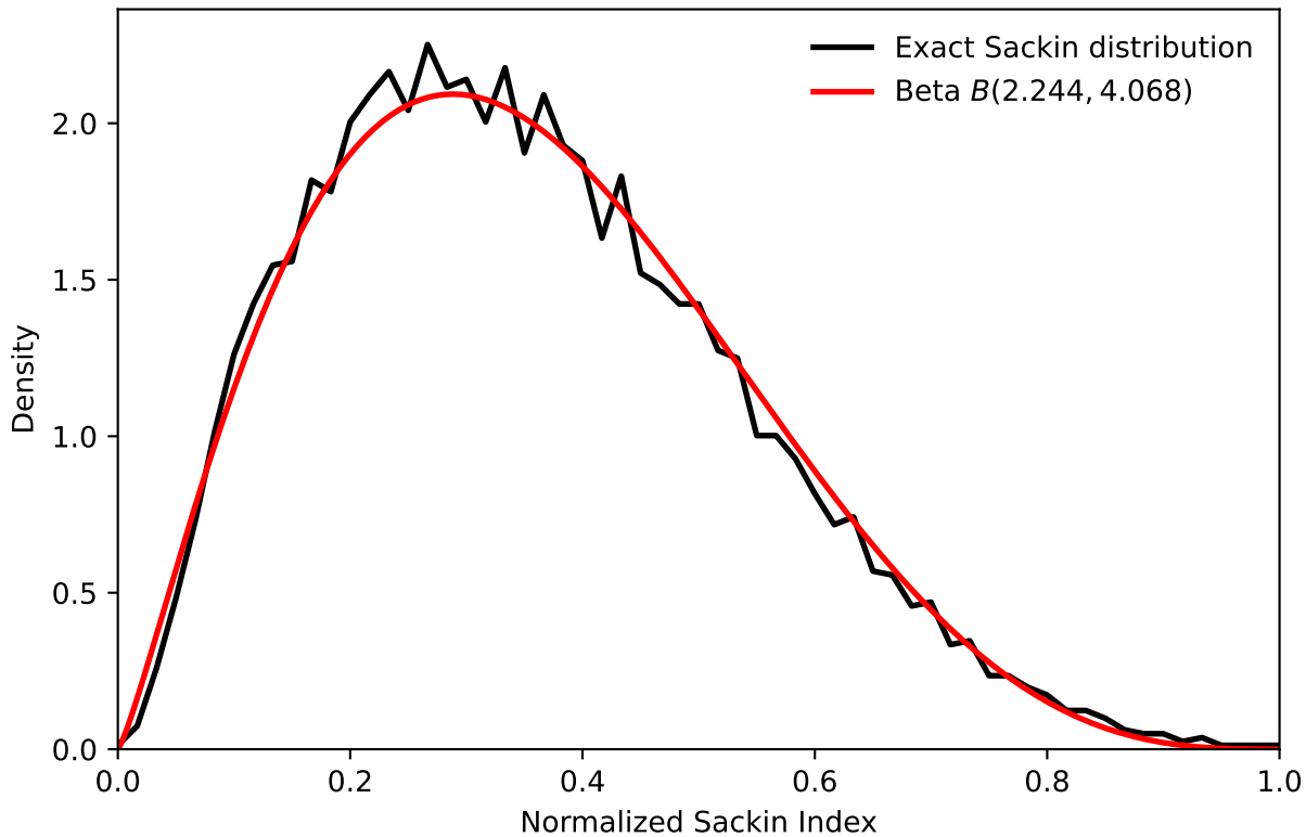
Sackin Index distribution for n = 15
