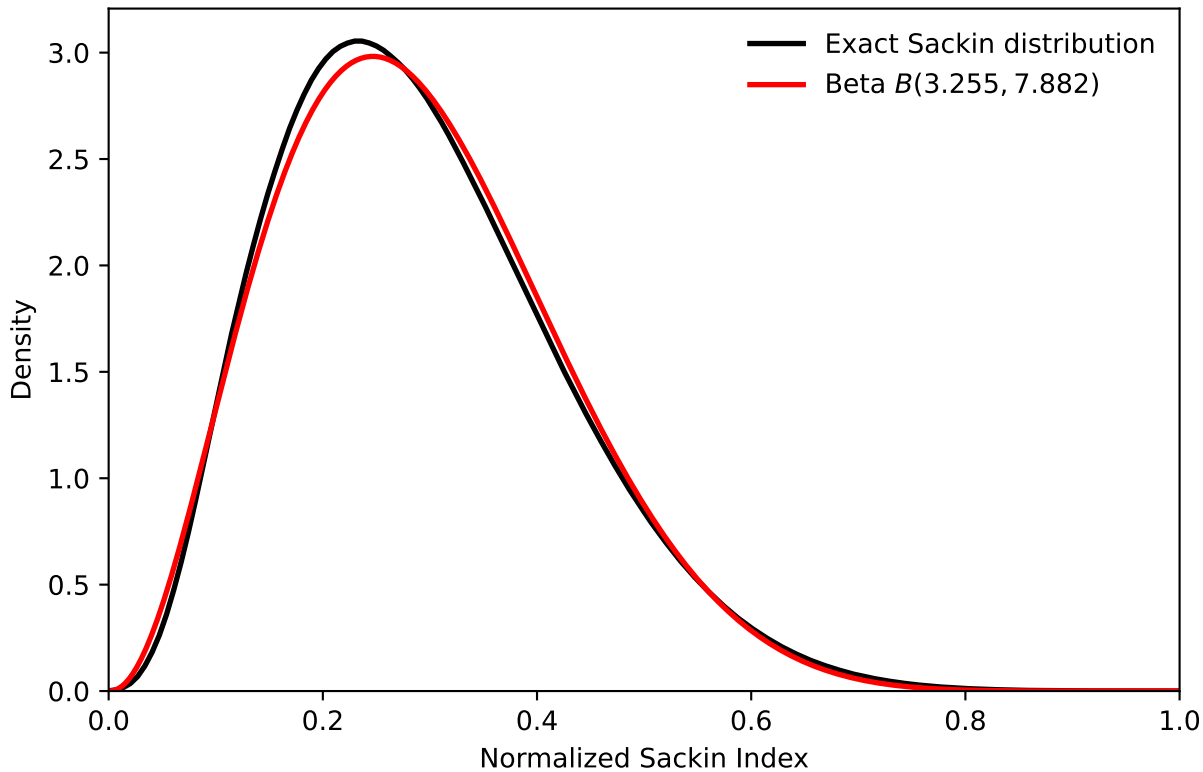
Full 3-ary trees, n = 41
