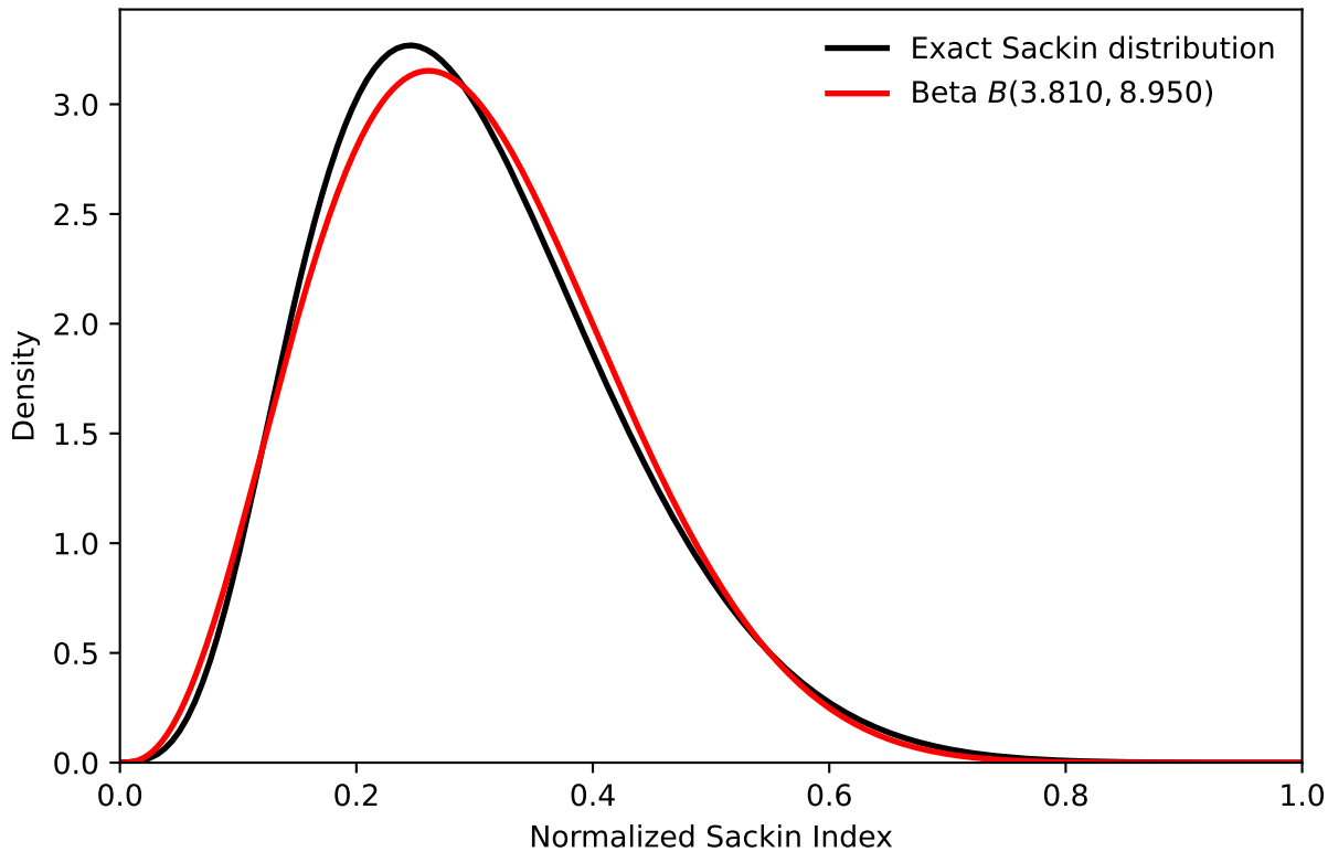
Full 6-ary trees, n = 101
