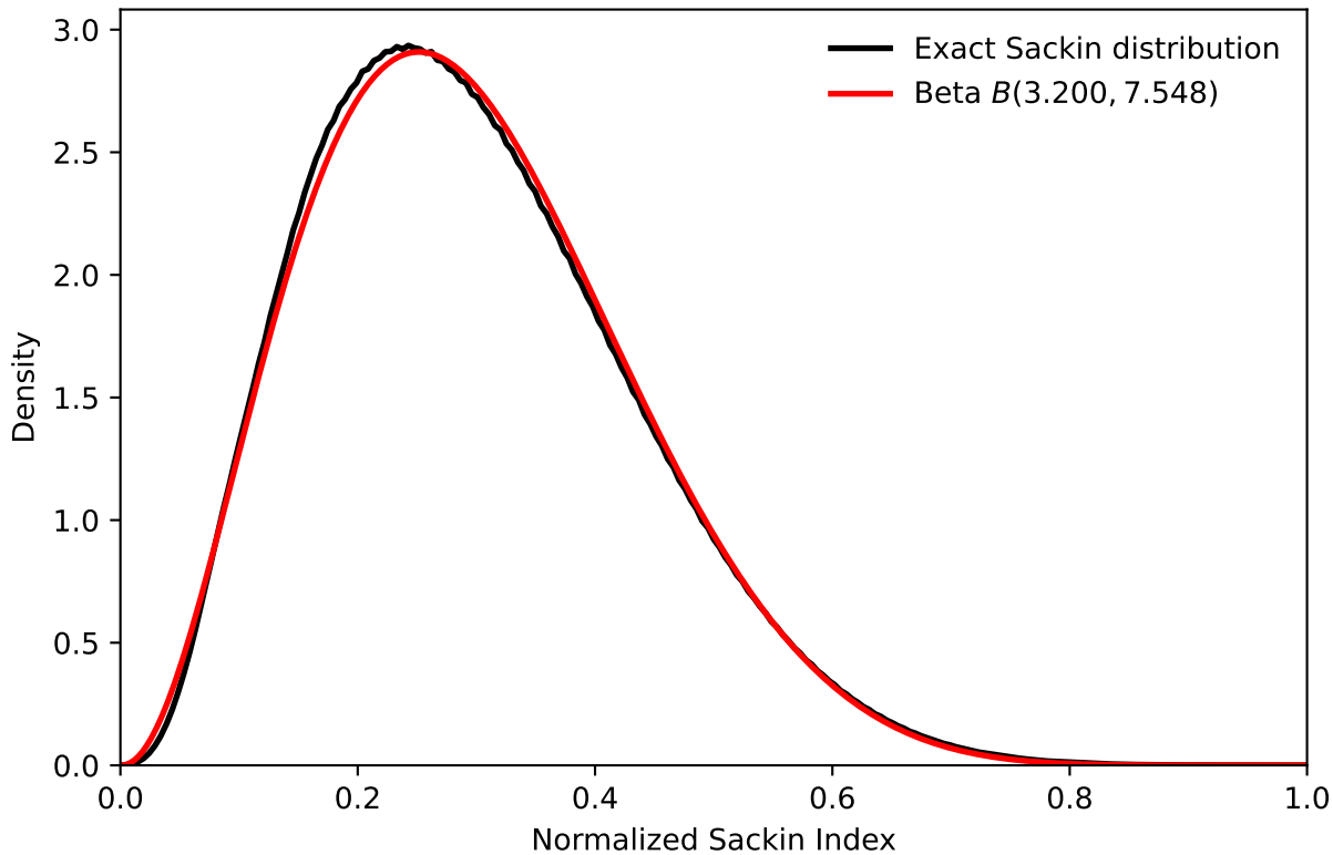
Sackin Index distribution for n = 25
