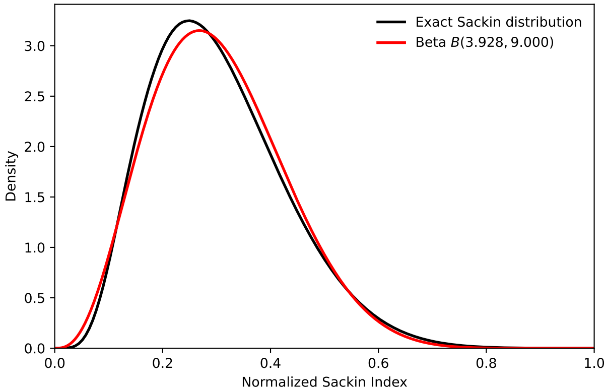
Full 4-ary trees, n = 61
