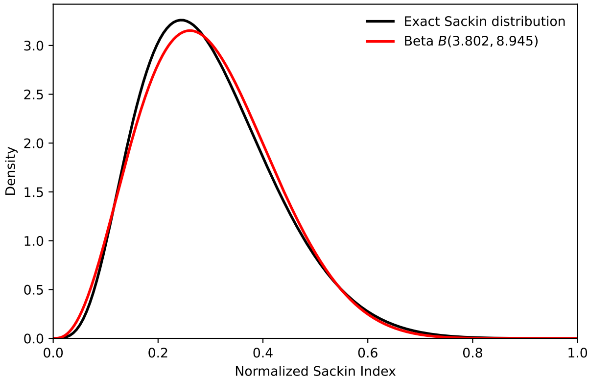
Full 5-ary trees, n = 81
