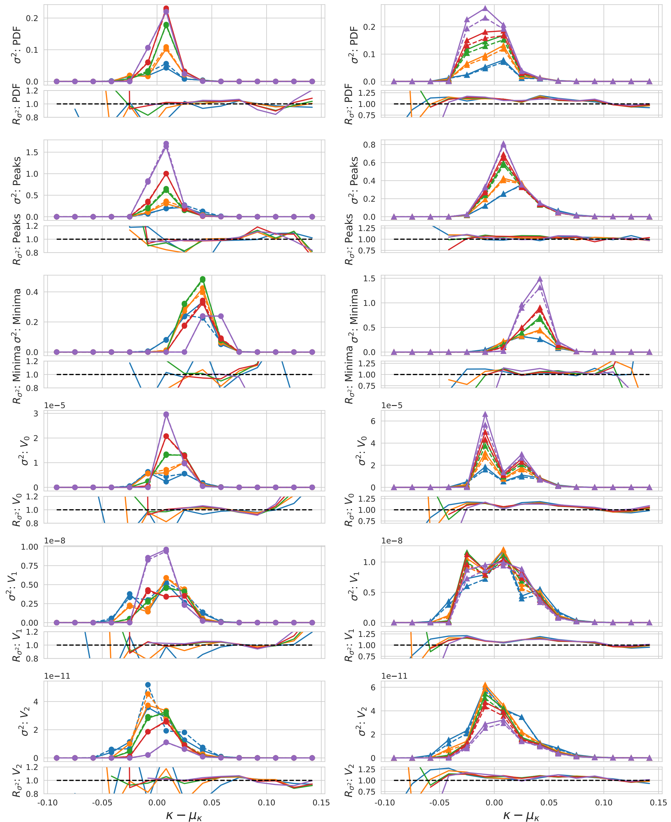
Variance \sigma^2 , and their ratio R_{\sigma^2} of Real-space Statistics for Multiple Noise Scales between TILED and BIGBOX at z_s = 0.5 (Left) and z_s = 1.5 (Right)
