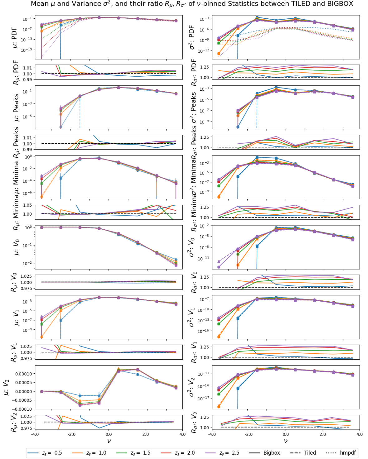
Figure 8.2: Comparison of the mean and variance for \nu -binned statistics, including the Minkowski Functionals ( V_0, V_1, V_2 ), the probability density function (PDF), and peak and minima counts. Results are derived from the BIGBOX and TILED simulations across source redshifts z_s = 0.5, 1.0, 1.5, 2.0 , and 2.5 , highlighting their sensitivity to super-sample effect. The figure illustrates how super-sample effect and other systematic effects influence the distribution and variance of these higher-order weak lensing statistics.
