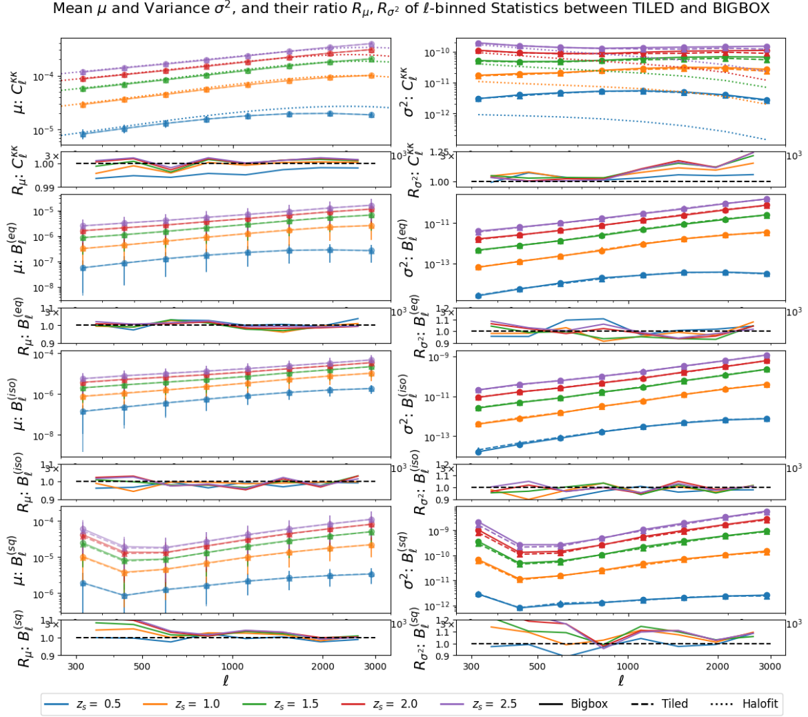
Figure 8.1: Comparison of the mean and variance for the angular power spectrum ( C_\ell^{KK} ) and the bispectrum components across three configurations: equilateral ( B_\ell^{(eq)} ), isosceles ( B_\ell^{(iso)} ), and squeezed ( B_\ell^{(sq)} ). Results are presented for the BIGBOX and TILED simulations across source redshifts z_s = 0.5, 1.0, 1.5, 2.0 , and 2.5 . The figure highlights how different simulation methodologies and super-sample effect influence the summary statistics of these cosmological observables.
