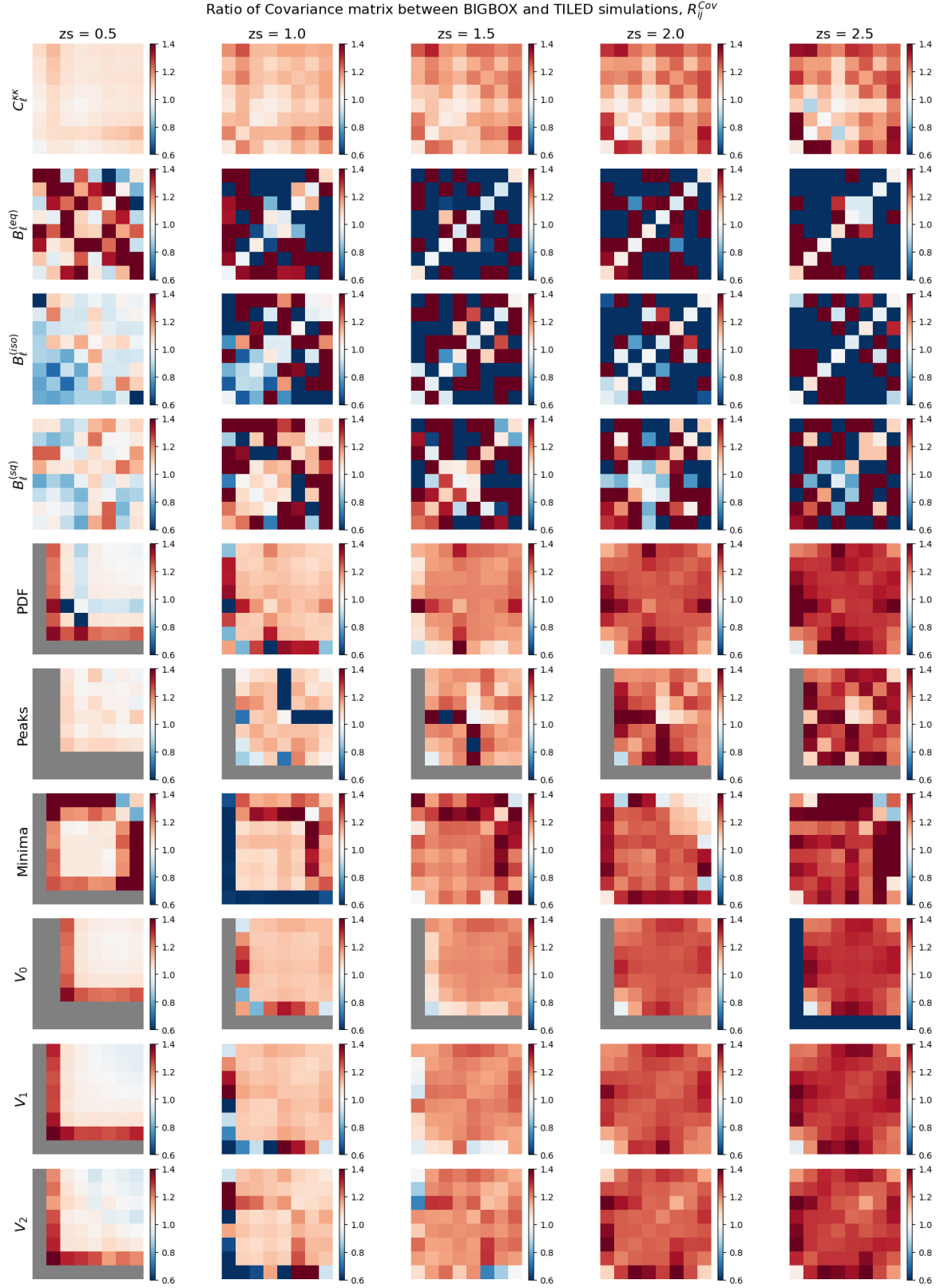
Figure 8.7: Ratios of covariance matrices ( R_{\text{Cov}} ) between the BIGBOX and TILED simulations across multiple source redshifts ( z_s = 0.5, 1.0, 1.5, 2.0 , and 2.5 ). The ratios consistently range from 10% to 30% above unity for most measured statistics, indicating the substantial impact of super-sample effect on the covariance structure.
