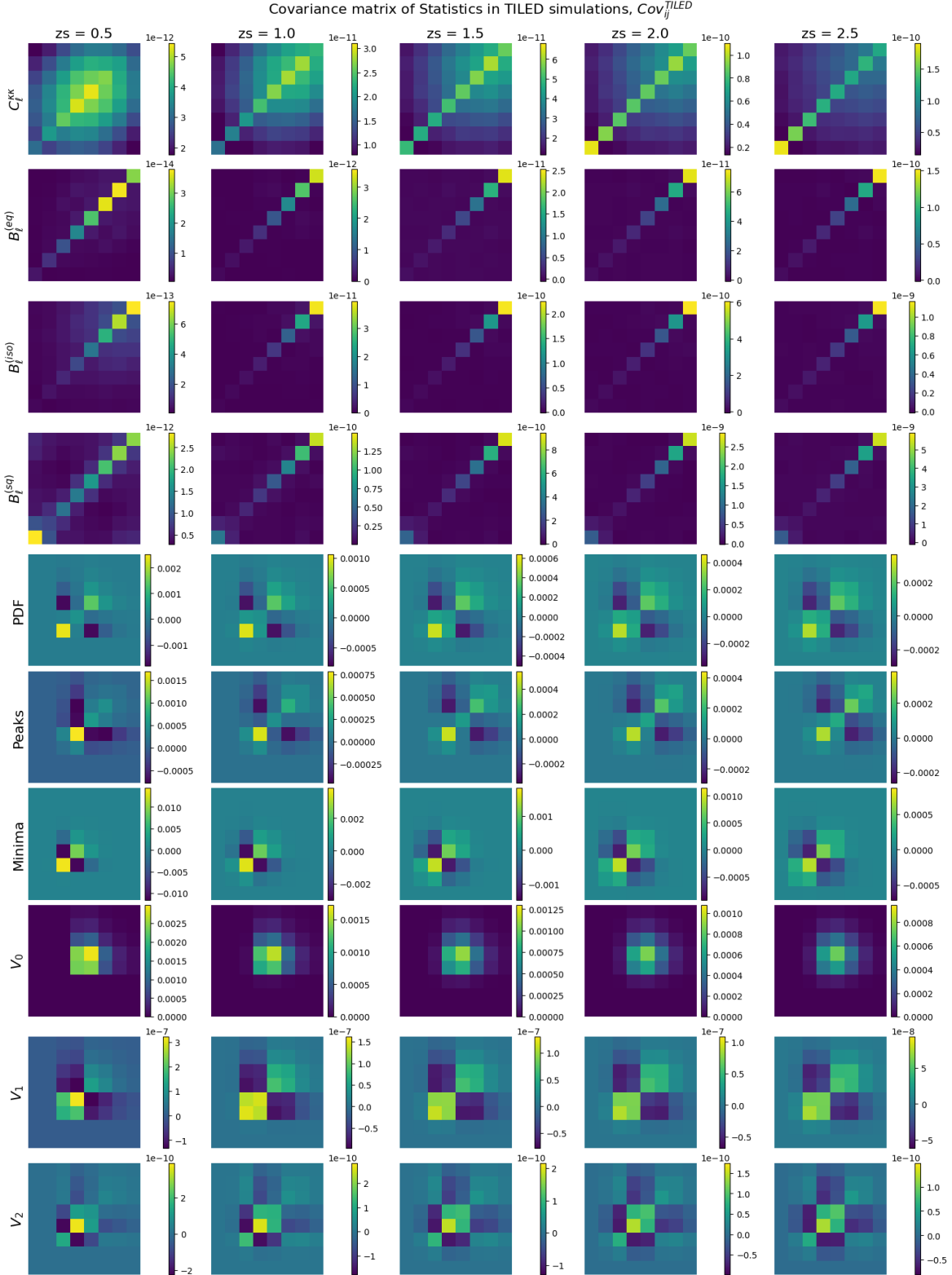
Figure 8.5: Covariance matrices of various summary statistics in the TILED simulations across multiple source redshifts ( z_s = 0.5, 1.0, 1.5, 2.0 , and 2.5 ), using a color scale consistent with Figure 8.4. These matrices demonstrate generally lower covariance values compared to the BIGBOX simulations, highlighting the reduced influence of super-sample effect due to the absence of larger-scale modes.
