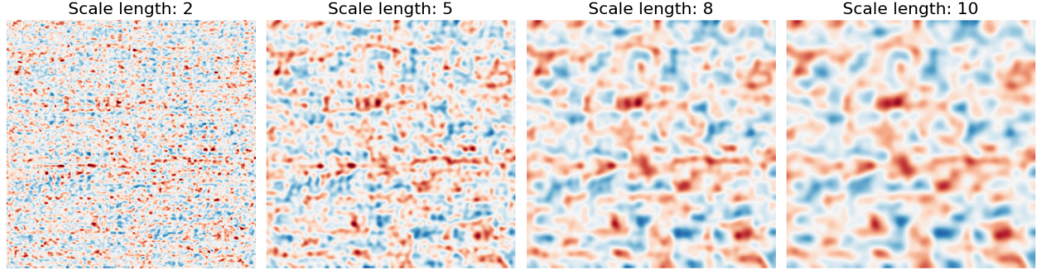
Figure 7.7: Effect of Gaussian smoothing on a noisy convergence map. Each panel shows the result of applying a Gaussian filter with a smoothing scale of \theta_G = 2', 5', 8', or 10' . As the smoothing scale increases, small-scale noise is progressively suppressed, making large-scale structures more prominent. This demonstrates how Gaussian smoothing effectively reduces shape noise while preserving the underlying lensing signal.
