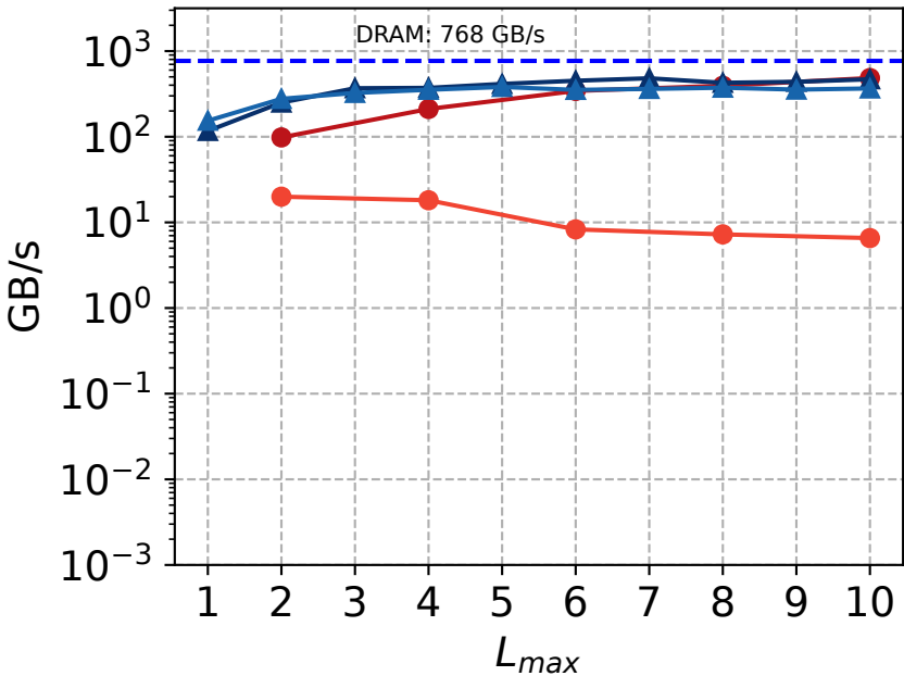
Average Bandwidth for SISO batch=10000
