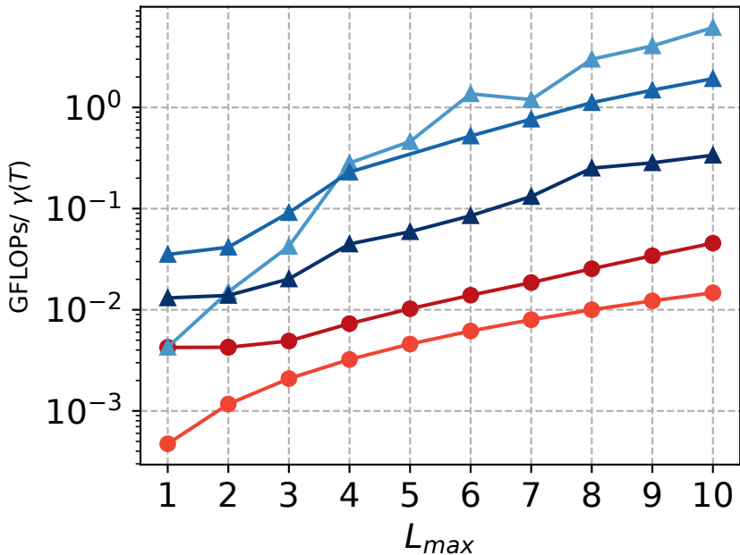
Total Normalized GFLOPs for MIMO batch=10000
