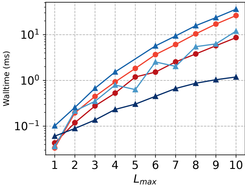
Forward Walltime (GPU) for MIMO batch=10000
