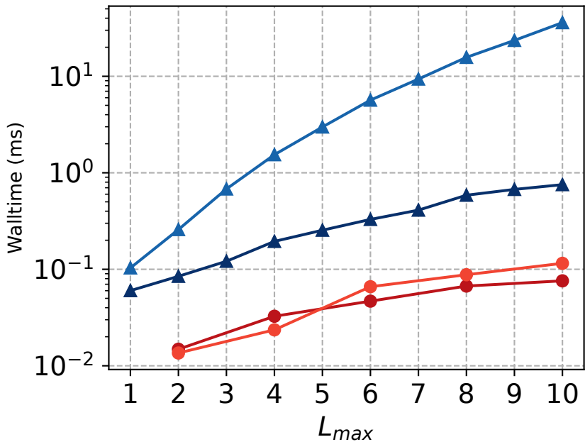
Forward Walltime (GPU) for SISO batch=10000
