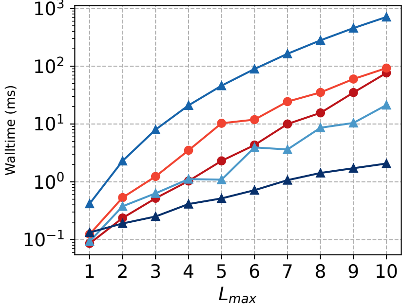
Backward Walltime (GPU) for MIMO batch=10000
