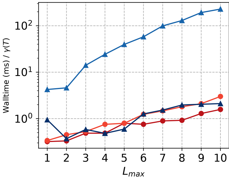
Total Normalized Walltime (CPU) for SIMO batch=10000
