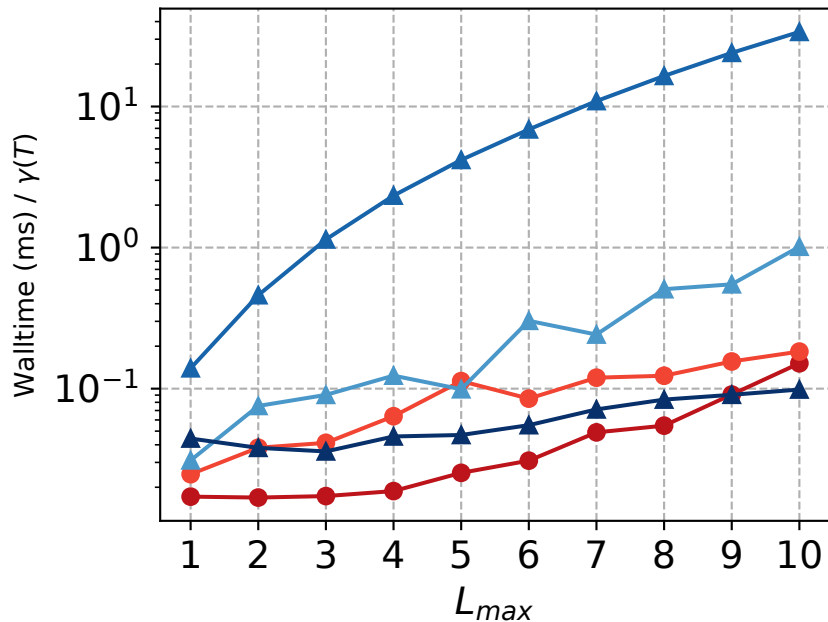
Backward Normalized Walltime (GPU) for MIMO batch=10000
