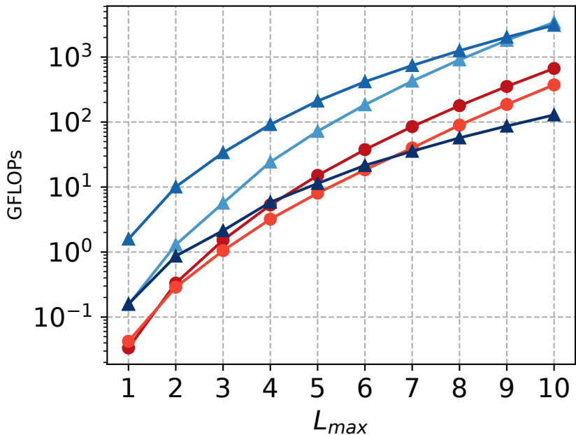
Total GFLOPs (Linux Perf) for MIMO batch=10000
