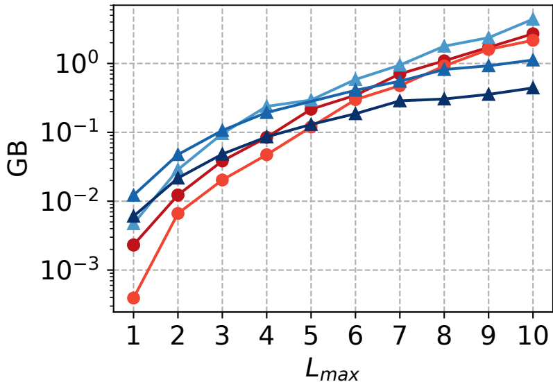
Total DRAM Read + Writes for MIMO batch=10000
