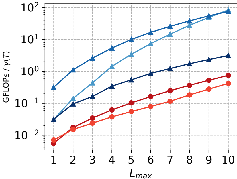
Total Normalized GFLOPs (Linux Perf) for MIMO batch=10000
