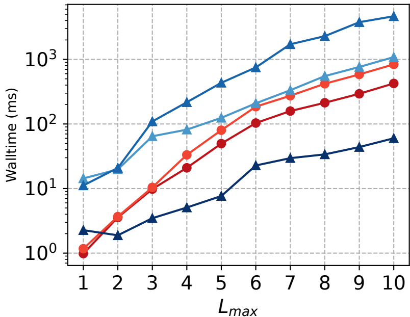
Total Walltime (CPU) for MIMO batch=10000
