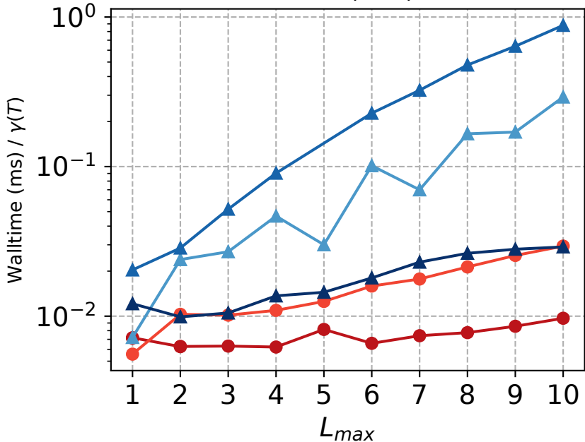
Forward Normalized Walltime (GPU) for MIMO batch=10000
