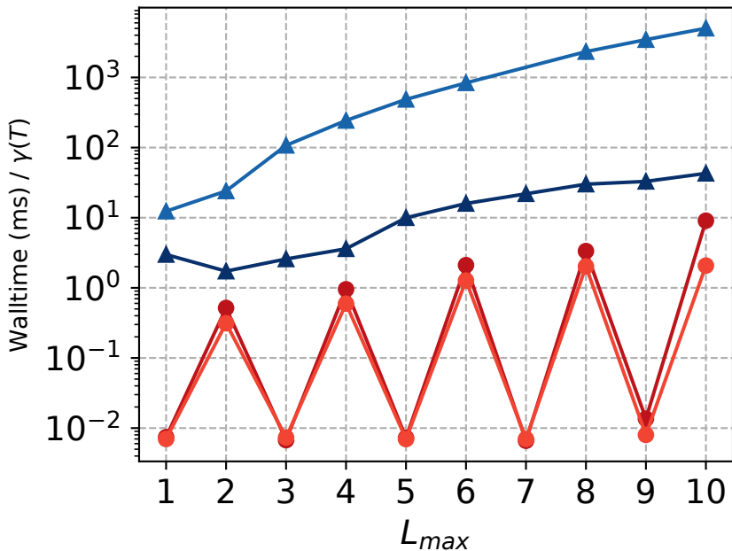
Total Normalized Walltime (CPU) for SISO batch=10000
