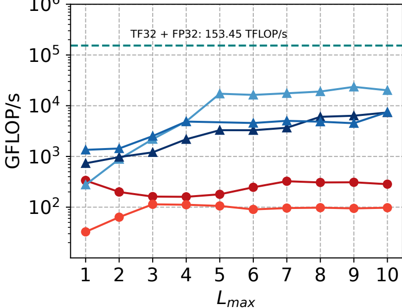
Average Throughput for MIMO for batch=10000
