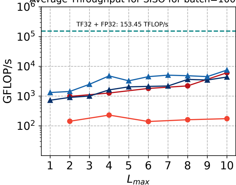
Average Throughput for SISO for batch=10000
