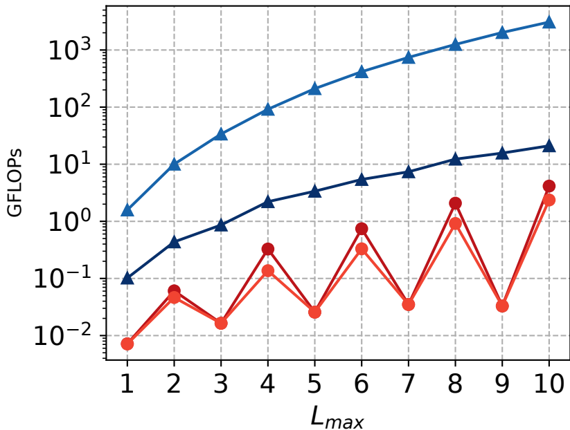
Total GFLOPs (Linux Perf) for SISO batch=10000
