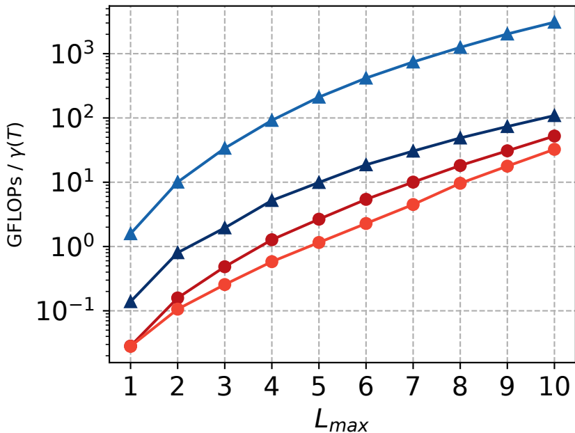
Total Normalized GFLOPs (Linux Perf) for SIMO batch=10000
