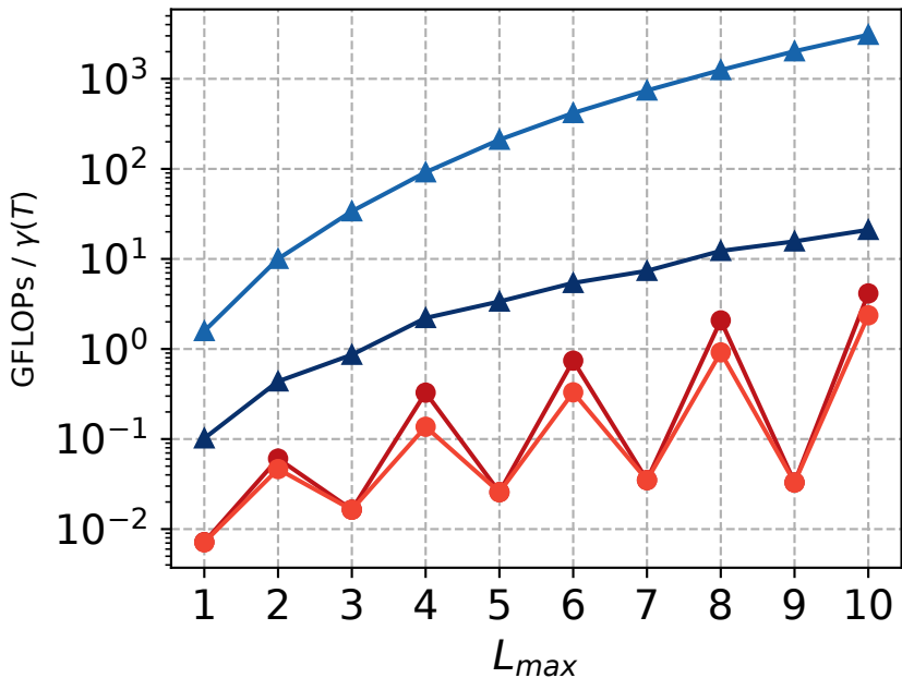
Total Normalized GFLOPs (Linux Perf) for SISO batch=10000
