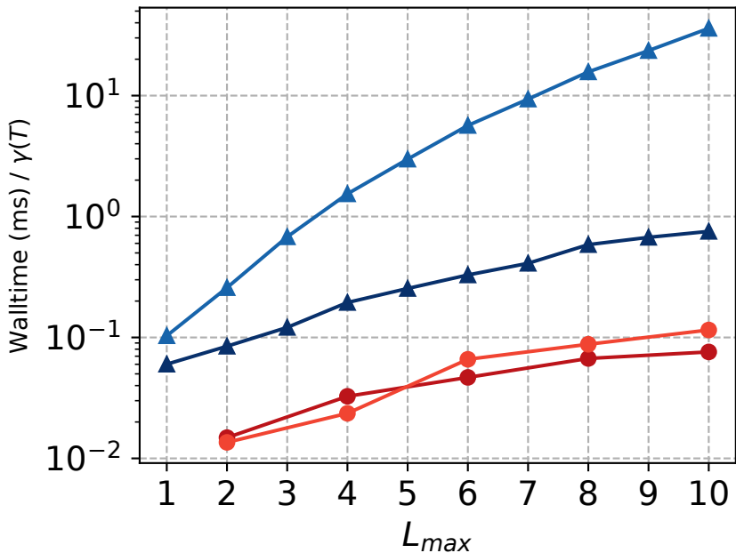
Forward Normalized Walltime (GPU) for SISO batch=10000
