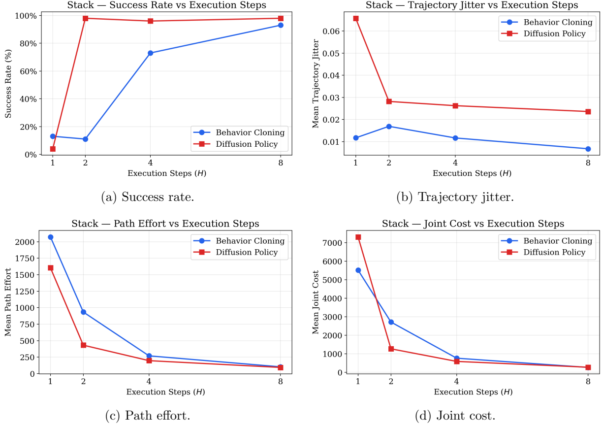
Figure 11: Behavior Cloning vs. Diffusion Policy on the Stack task across execution horizons H \in \{1, 2, 4, 8\} , for each of the four evaluation metrics.
