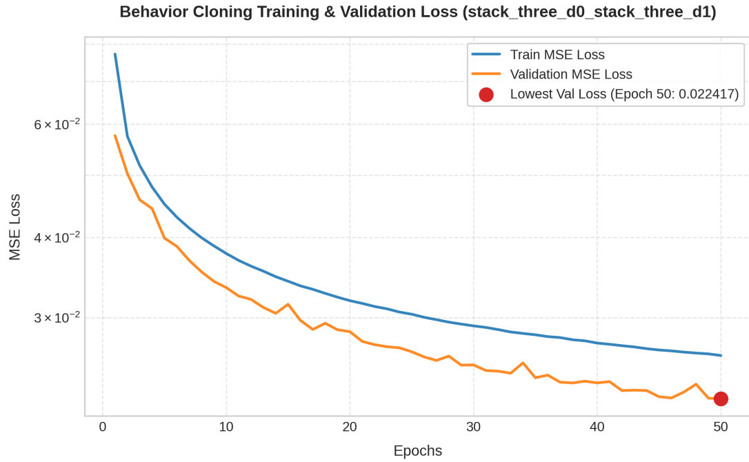
Figure 5: Training and validation Mean Squared Error (MSE) loss curves on a log scale for the Behavior Clone model.
