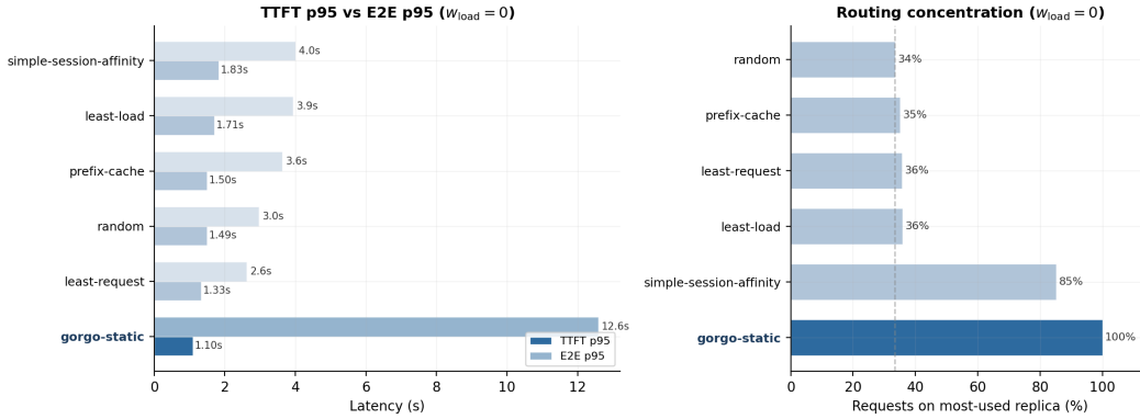
Figure 4: Left : TTFT p95 (dark) vs. E2E p95 (light) on the midday diurnal trace with w_{\text{load}}=0 . gorgo-static wins TTFT but its E2E inflates to 12.6 s. Right : routing concentration. gorgo-static sends 100% of requests to one replica.
