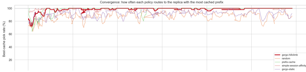
Figure 2: Best-cache-pick rate over the W1 tuning window for five policies. gorgo-hillclimb (red) converges to ~95–100% within the first few minutes; baselines either oscillate or stay flat at lower rates.
