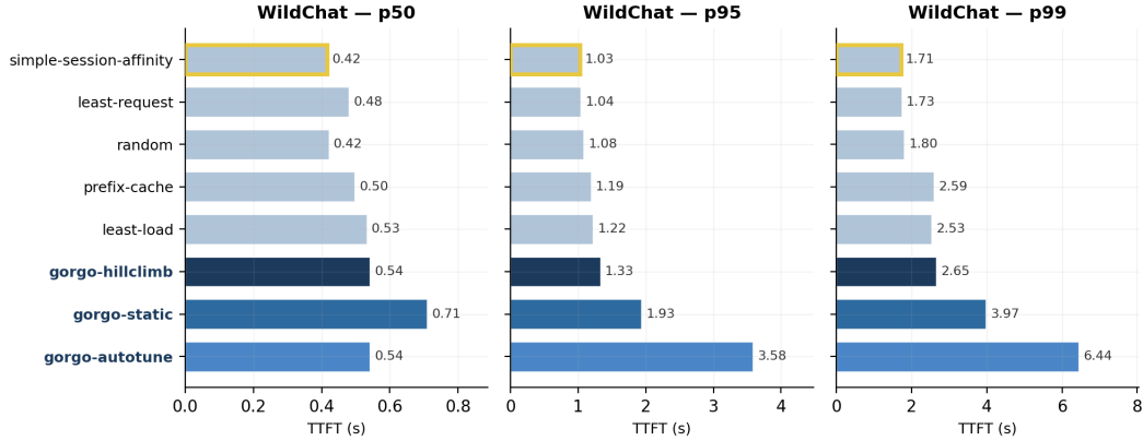
Figure 7: WildChat-4.8M replay, per-percentile TTFT (p50/p95/p99) across the eight policies. GORGO variants (dark blues) are not competitive: gorgo-static and gorgo-autotune are the slowest two policies at the tail, and gorgo-hillclimb sits mid-pack. The ranking inverts the ARTChat-411k result, consistent with the regime argument in §2.
