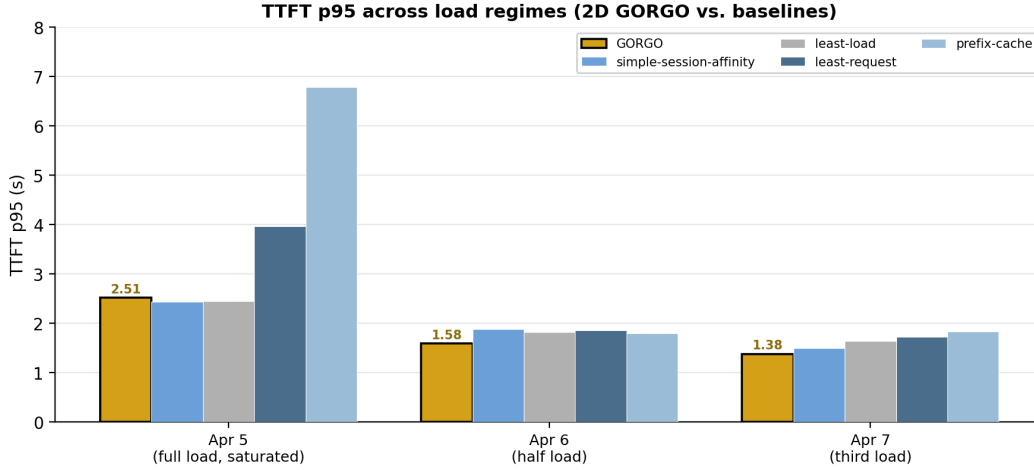
Figure 3: TTFT p95 across the three load-sweep windows (Table 2), GORGO (gold) vs. baselines under the frozen 2D weights. At full load (Apr 5, saturated) GORGO is within 3.5% of the best baseline; as load backs off to half (Apr 6) and a third (Apr 7) of capacity, GORGO becomes the lowest-p95 policy in every window, the advantage widening as the fleet gains slack.
