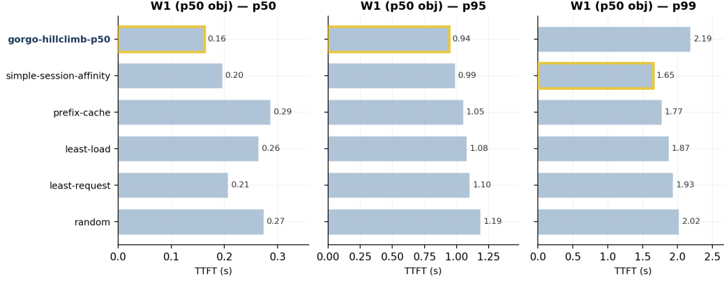
Figure 5: W1 TTFT with p50 objective. gorgo-hillclimb (gold outline) achieves the best p50 (0.163 s) by prioritizing RTT over cache.
