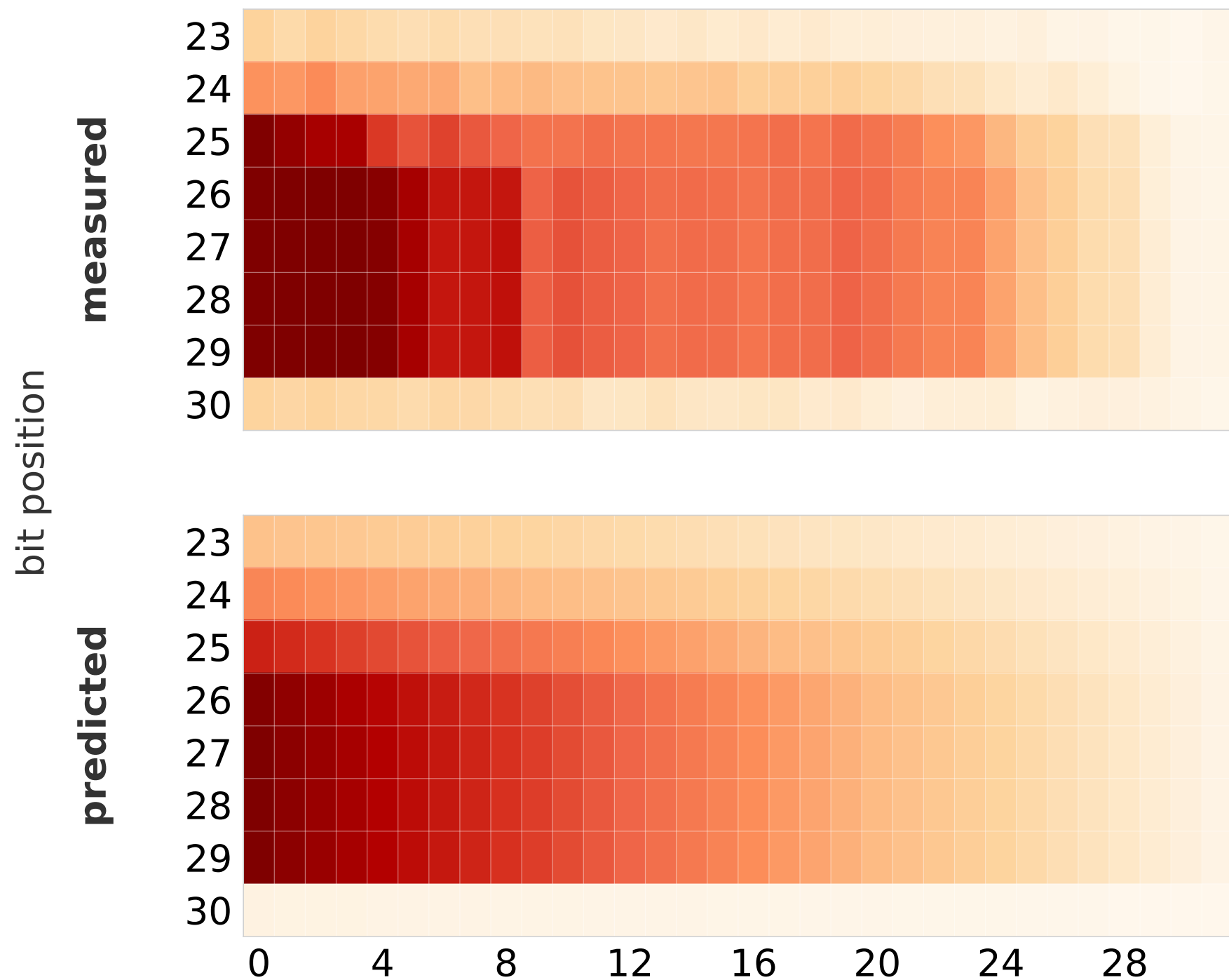
stuck-at-0 \rho = 0.941
