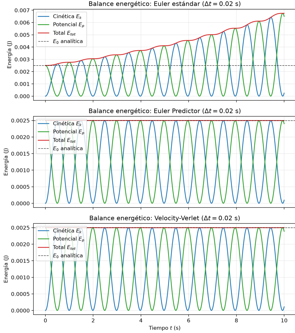
Figure 6: Kinetic, potential, and total energy evolution at \Delta t = 0.02 s. Top: Standard Euler. Middle: Euler Predictor. Bottom: Velocity-Verlet.
