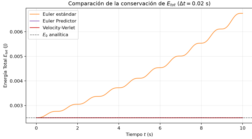
Figure 7: Comparison of total mechanical energy E_{tot}(t) conservation between standard Euler, Euler Predictor, and Velocity-Verlet at \Delta t = 0.02 s.
