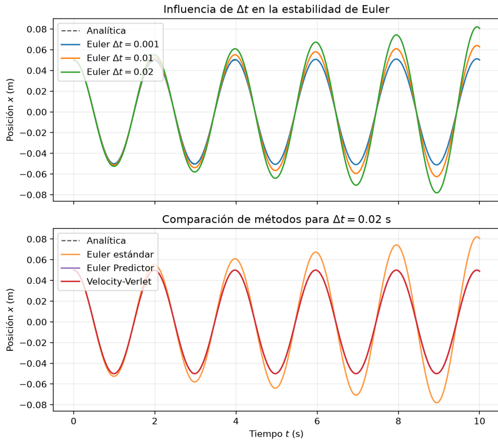
Figure 4: Oscillator position x(t) over time. Top: Influence of \Delta t \in \{0.001, 0.01, 0.02\} s on the standard Euler method. Bottom: Comparison between standard Euler, Euler Predictor, and Velocity-Verlet for \Delta t = 0.02 s against the analytical solution.
