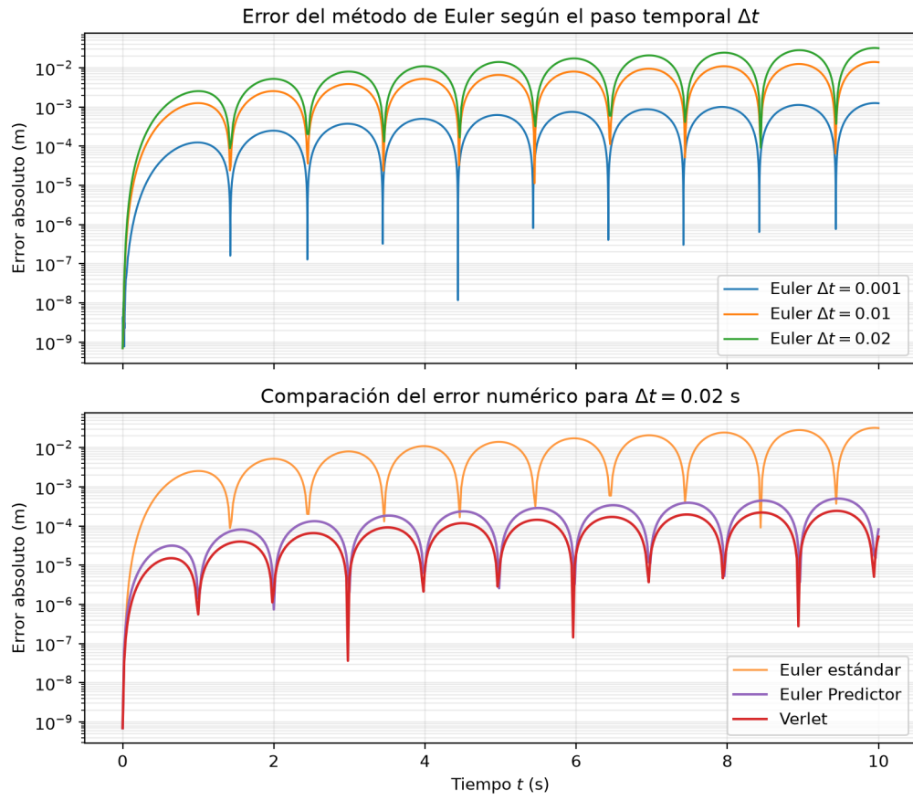
Figure 5: Absolute error in position |x_{\text{num}} - x_{\text{exact}}| (logarithmic scale). Top: Error in Euler's method as a function of \Delta t . Bottom: Numerical error comparison among the three algorithms for \Delta t = 0.02 s.
