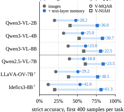
(a) images \rightarrow memory ( \Delta , pp), six readers
