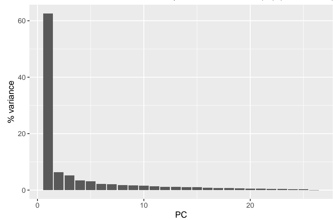
Data_To_Clean_Soluble – Group — PCA variance (%) (after_norm)
