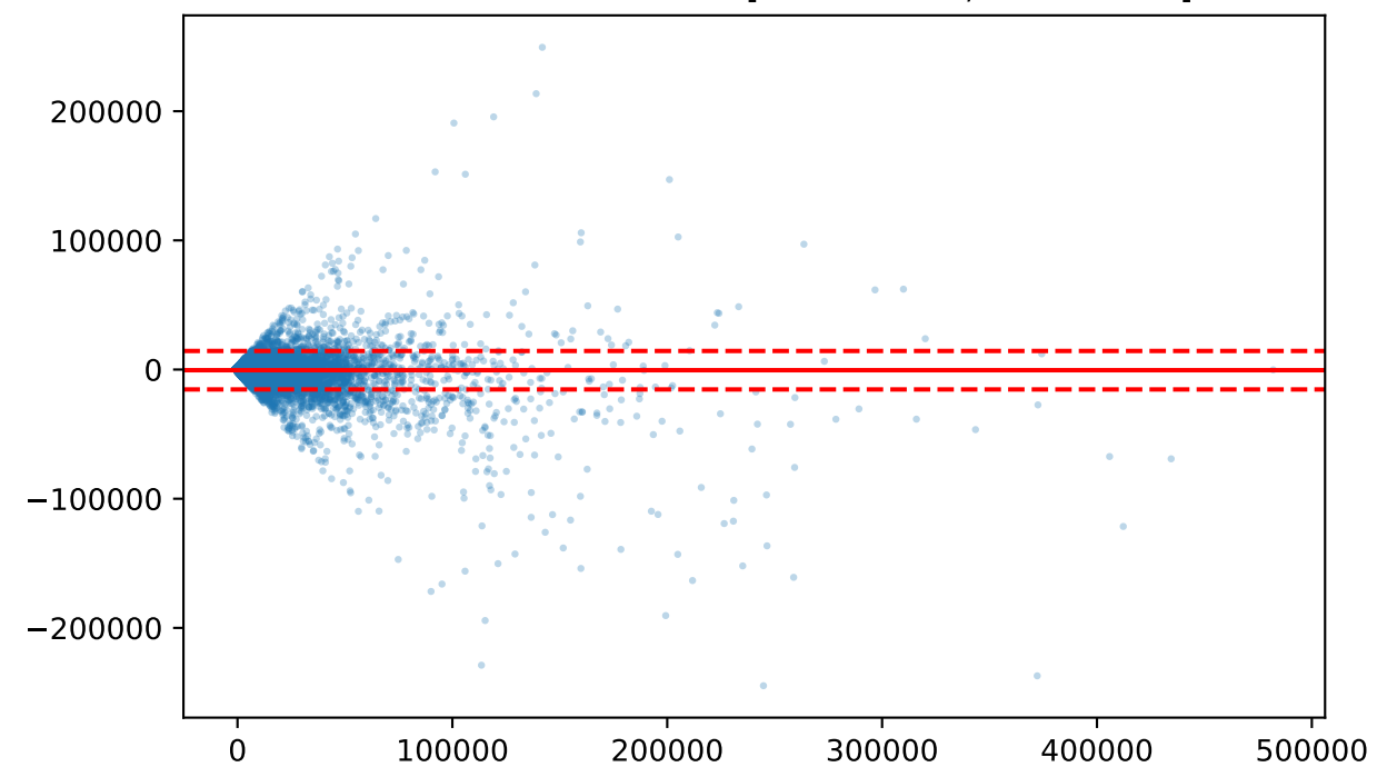
BA Bias=-504.865 LoA=[-15397.400, 14387.671]
