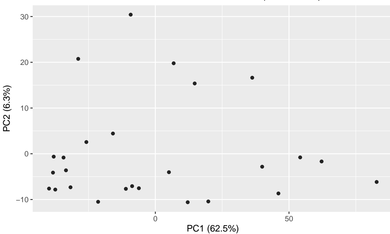
Data_To_Clean_Soluble – Time — PCA scores (after_norm)
