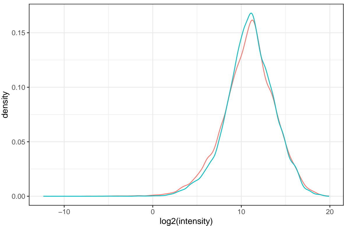
Pooled intensity distributions
