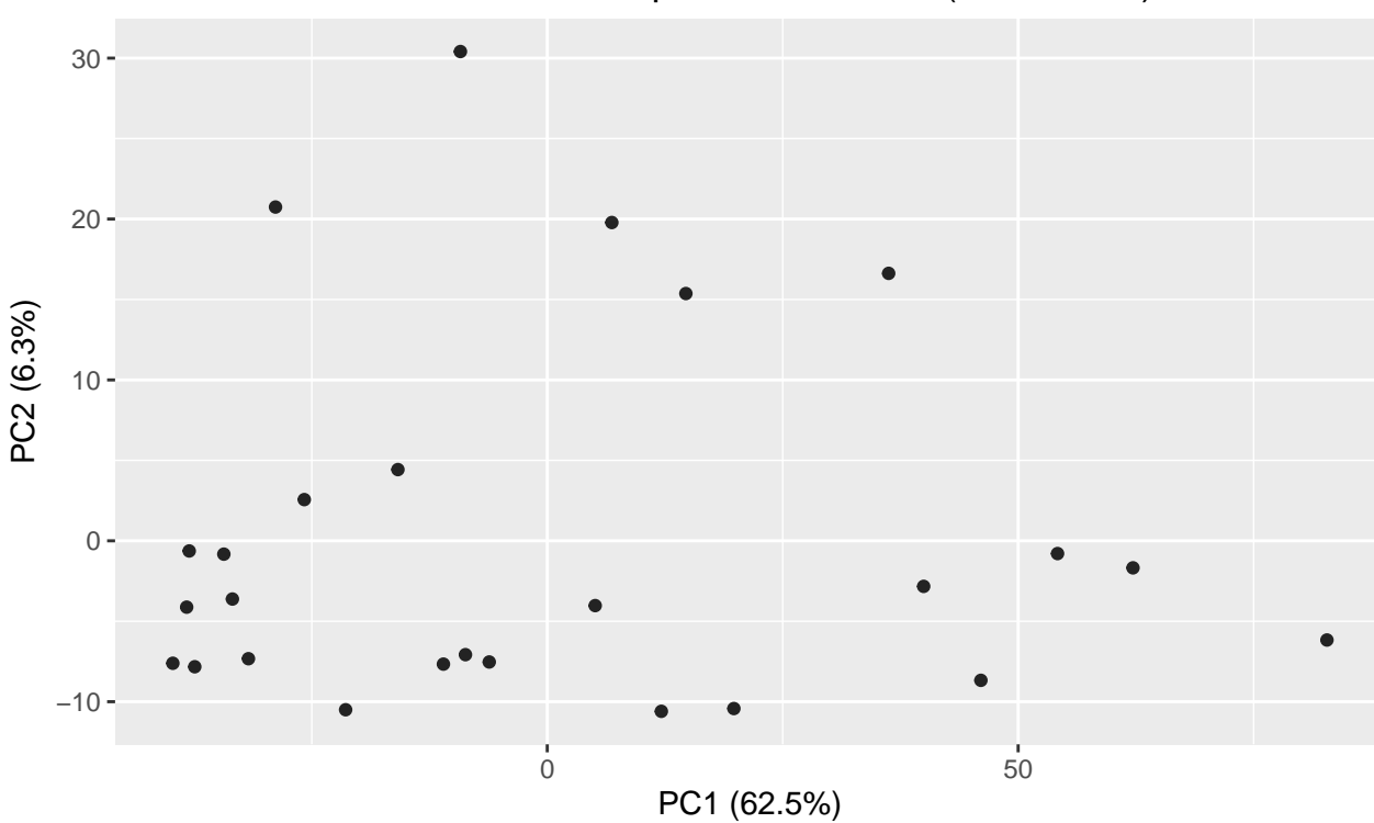
Data_To_Clean_Soluble – Group — PCA scores (after_norm)
