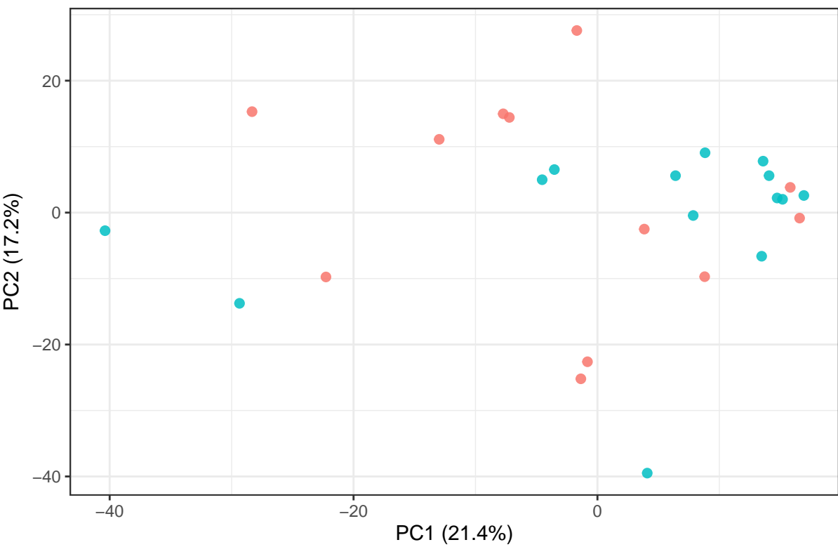
PCA scores (cleaned matrix)
