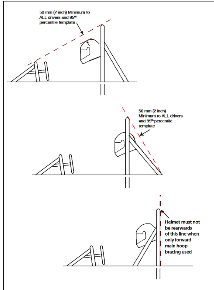
Figures from Top: 4a, 4b, and 4c- Roll Hoops and Helmet Clearance
