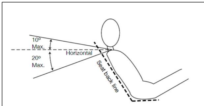
Figure 20 - Shoulder Harness Mounting – Side View
