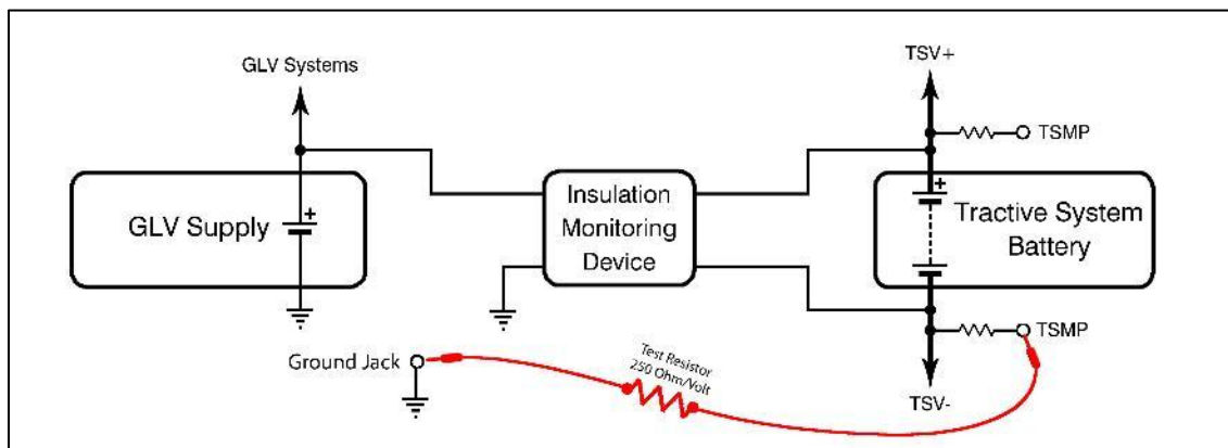
Figure 43 – Insulation Monitoring Device Test
