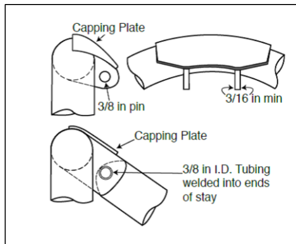
Figure 8 – Double-Lug Joint
