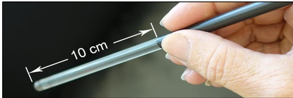
Figure 33 - Finger Probe
