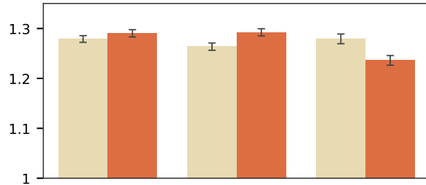
IRT Discrimination
