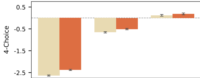
IRT Difficulty
