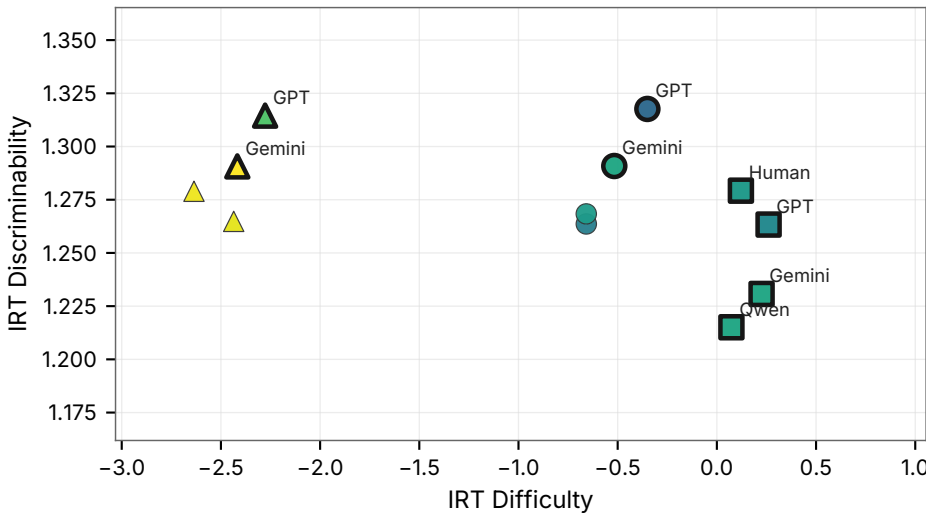
MCQ Generation
