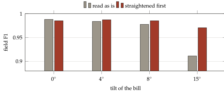
Figure 12: Field F1 on 100 tilted generated bills, with and without straightening.
