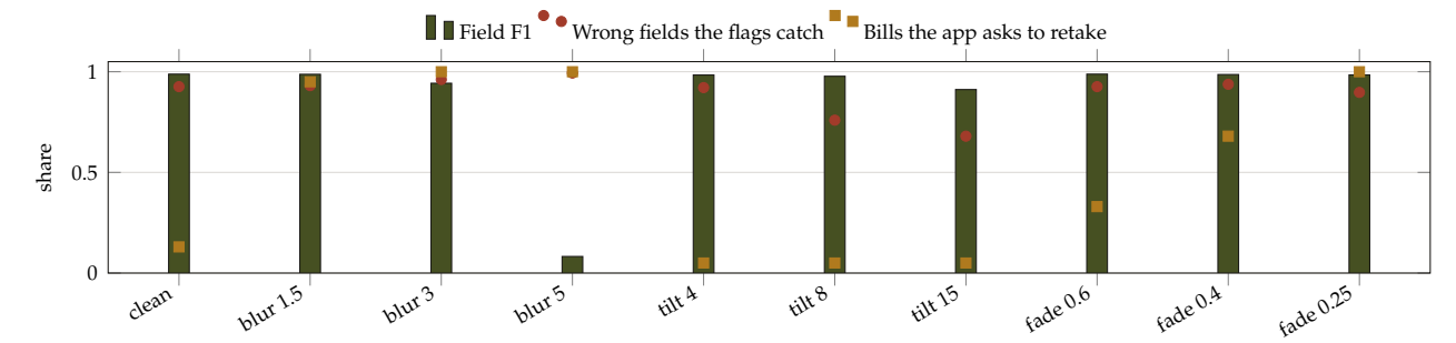
Figure 7: Controlled degradation of 100 unseen generated bills.
